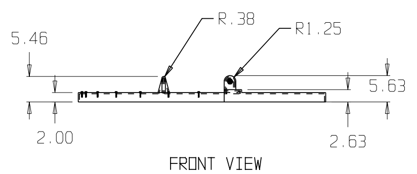
COMPLETE HINGED LID ASSEMBLY FOR A 48" DIA. TANK (AFTER TRIMMING)
