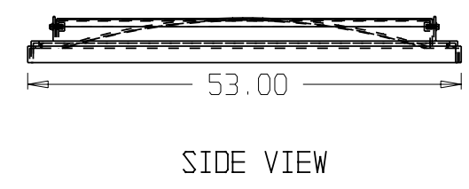
COMPLETE HINGED LID ASSEMBLY FOR A 48" DIA. TANK (AFTER TRIMMING)
